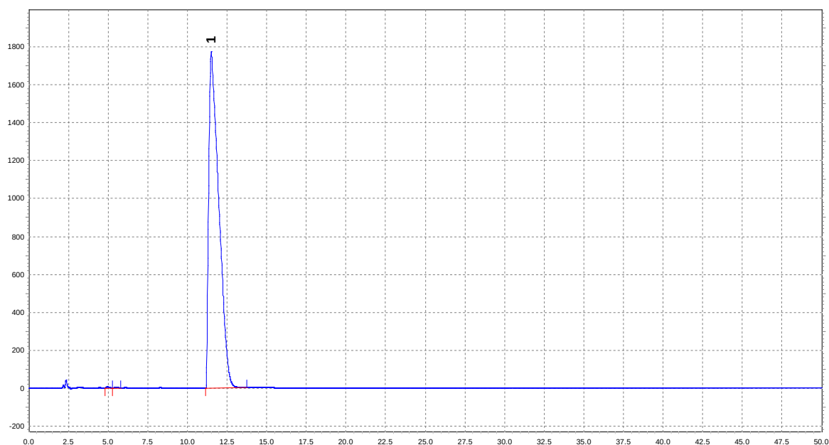
Peak ID: 1: Trospium
