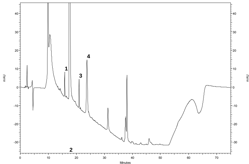
Peak ID: 1: Impurity D; 2: Lorazepam; 3: Impurity B; 4: Impurity E
