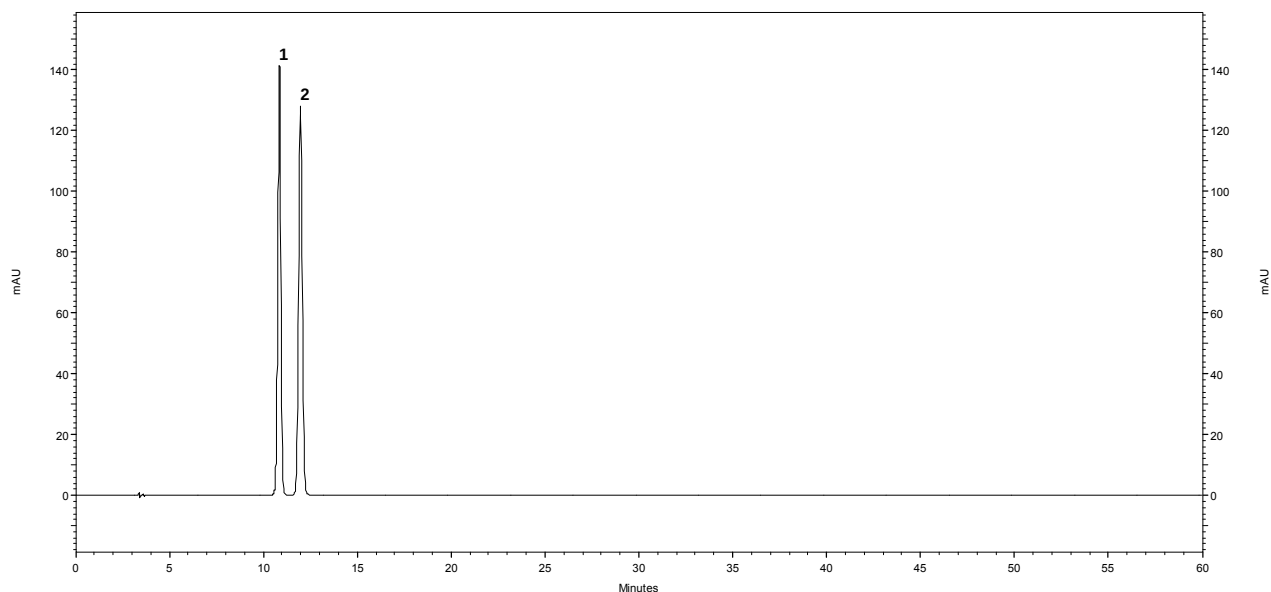
Peak ID: 1: Dihydrocodeine tartrate; 2: Codeine phosphate.
