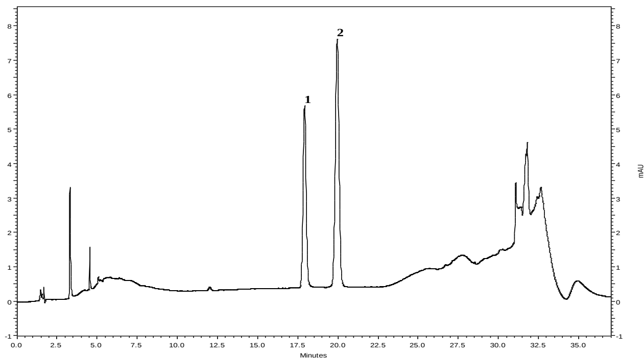
Peak ID: 1: Codeine; 2: 4'-chloroacetanilide
