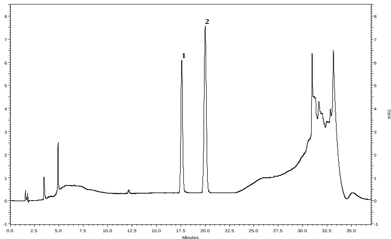
Peak ID: 1: Codeine; 2: 4'-chloroacetanilide
